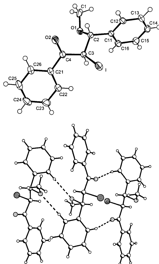
Figure 1. Top: An ORTEP picture of 3c , drawn with 50% probability displacement ellipsoids and with hydrogen atoms shown as arbitrarily sized spheres. Bottom: The molecules in 3c are associated by weak hydrogen bonding interactions into infinite chains that propagate along the b axis. Each molecule is linked to two neighbouring ones: to one through a pair of hydrogen bonds formed between carbonyl oxygens and phenyl protons, with lengths O(2)\cdots C(12)^i = 3.289(3) Å ((i) 2 -x, 1 -y, 1 -z ), and to another through a pair of hydrogen bonds formed between methoxy oxygens and phenyl protons, with lengths O(1)\cdots C(16)^{ii} = 3.434(3) Å ((ii) 2 -x, -y, 1 -z ).
